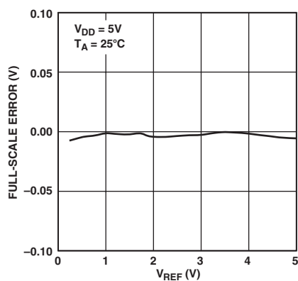
TPC 22. Full-Scale Error vs. V_{REF} (Buffered)
