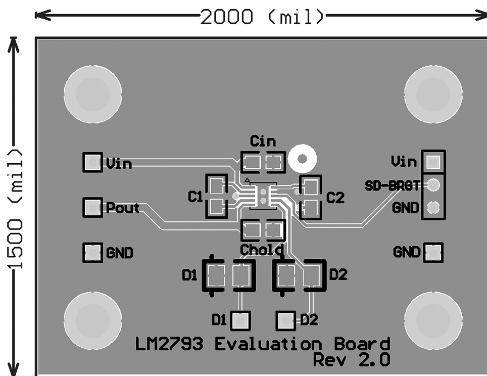
Figure 1. Top Layer, Top View
