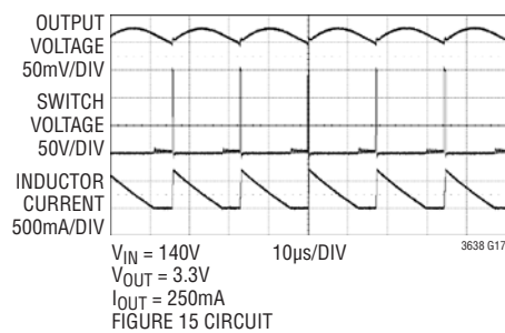
Operating Waveforms, V_{IN} = 140V
