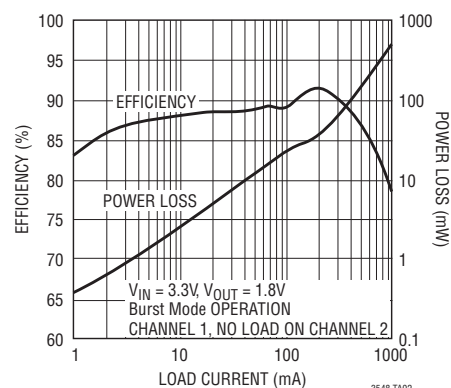
LTC3548 Efficiency Curve
