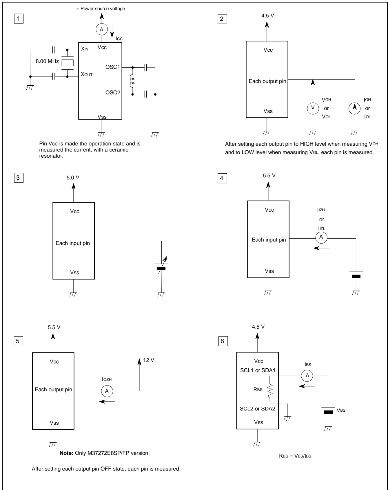
Fig.12.1 Measure Circuits
