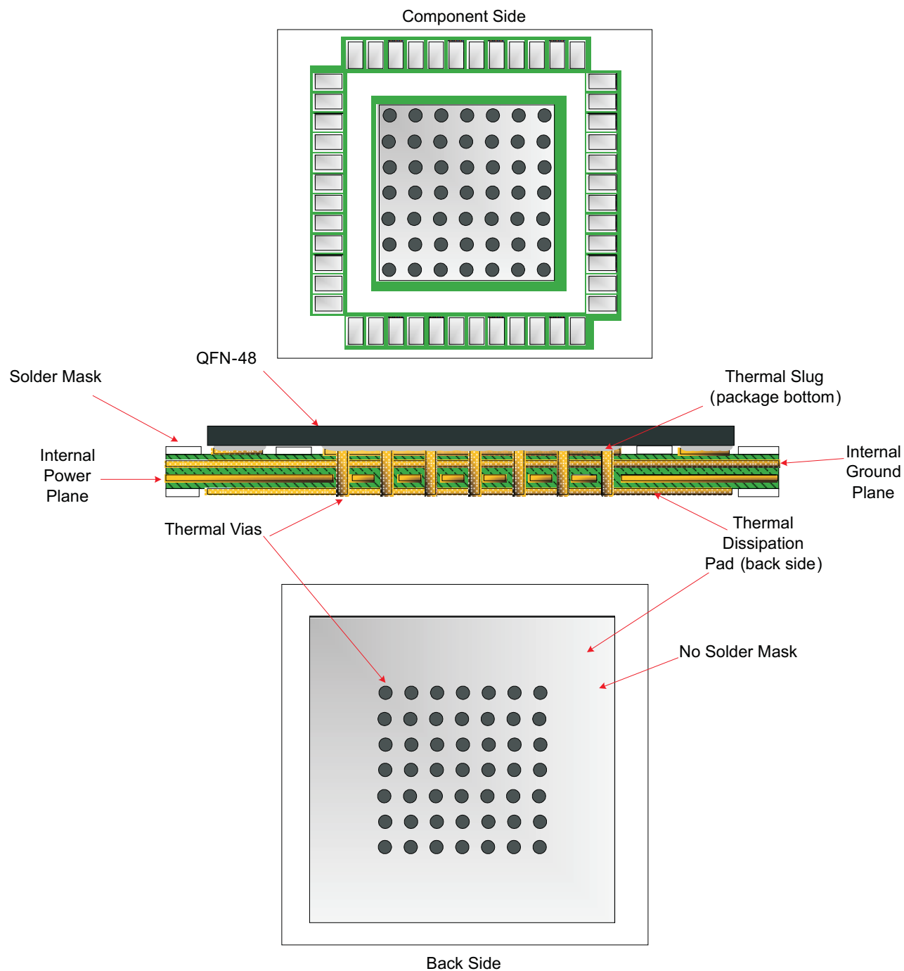
Figure 28. CDCE18005 Recommended PCB Layout
