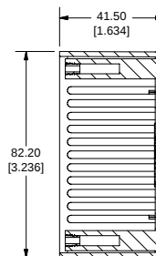
SECTION B-B
