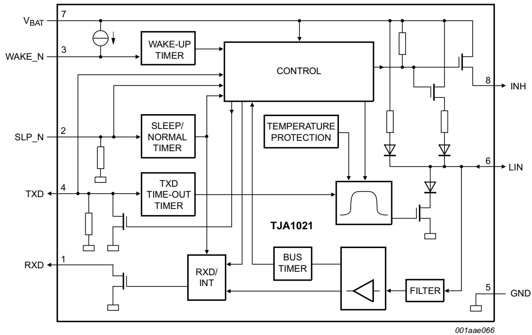
Fig 1. Block diagram
