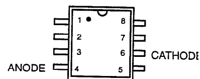
8 Lead SOIC (0.150")
