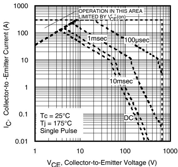
Fig. 4 - Forward SOA
