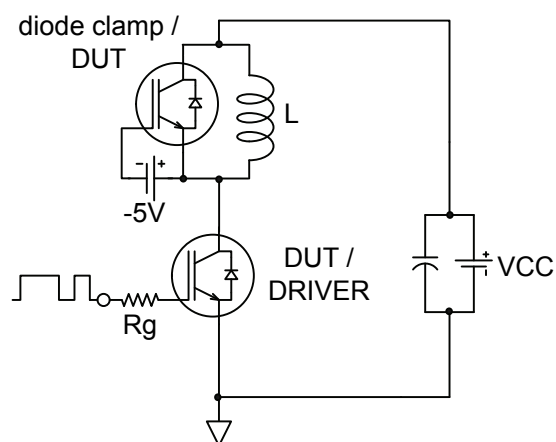
Fig.C.T.2 - RBSOA Circuit
