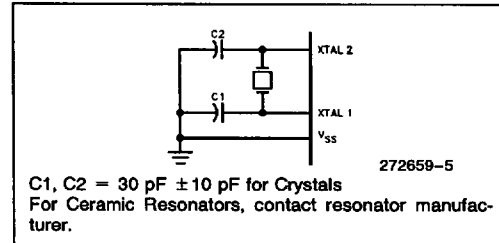
Figure 3. Oscillator Connections
