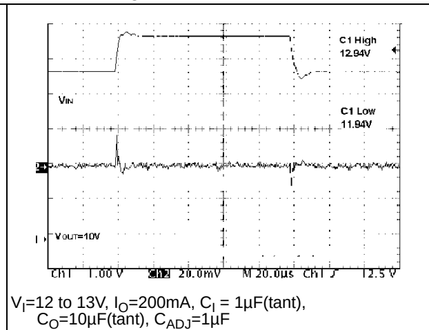
Figure 21. Line transient
