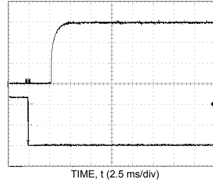
Figure 22. Typical Start-Up Using Remote On/Off, negative logic version shown.
