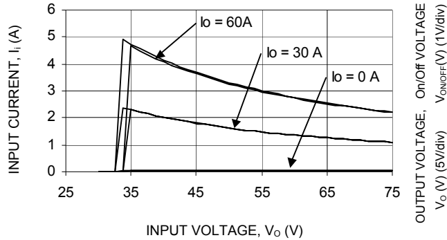
Figure 7. Typical Input Characteristic at Room Temperature.
