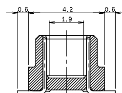
SECT. D-D
