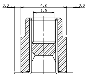
SECT. D-D
