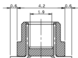
SECT. D-D
