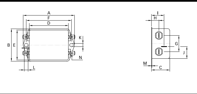
Connection style -06, 16 and 20 A types
