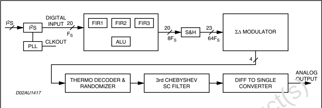
Figure 1. Block diagram
