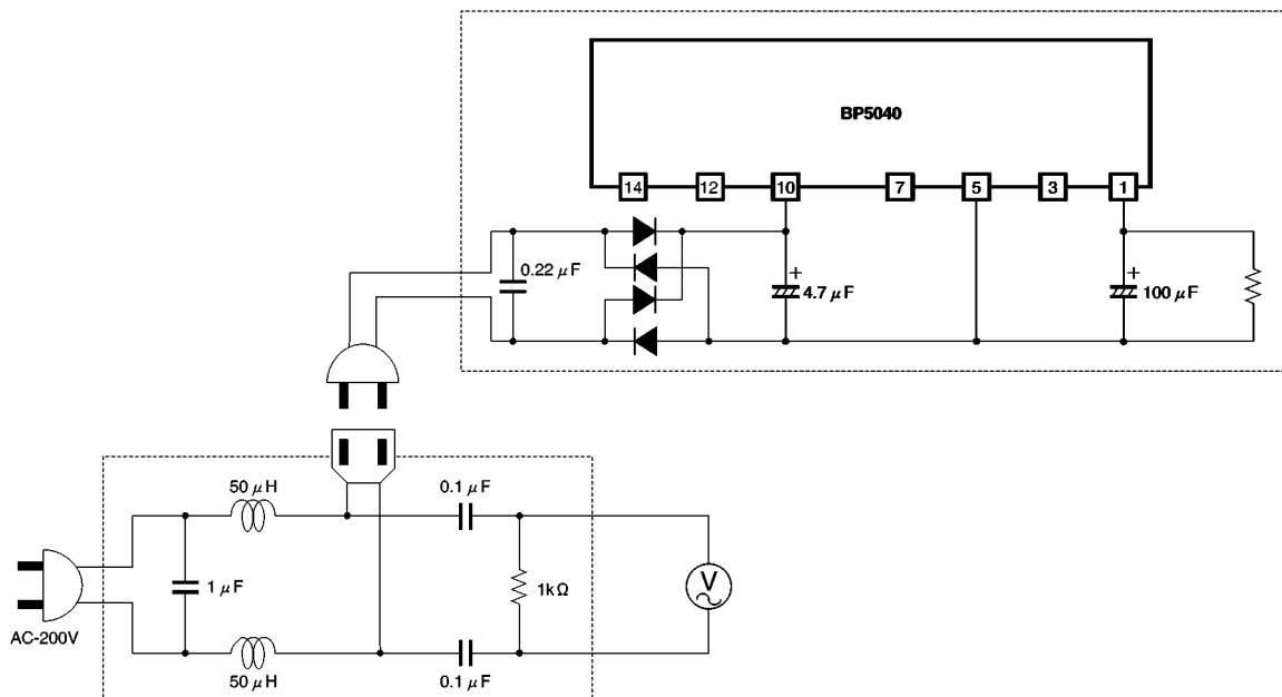
Fig.6 Test circuit
