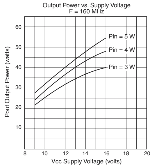
Figure 7. Power Output vs Supply Voltage (160 MHz)
