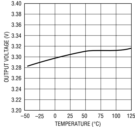
LT1573-3.3V Output Voltage vs Temperature
