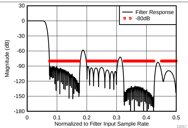
Figure 36. Decimate by 4 - Stopband Response
