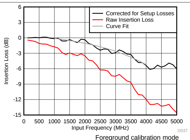
Figure 32. Insertion Loss vs Input Frequency
