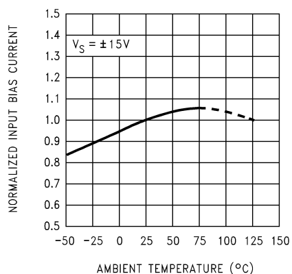
Normalized Input Bias Current vs Ambient Temperature
