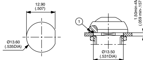
① - O-ring
