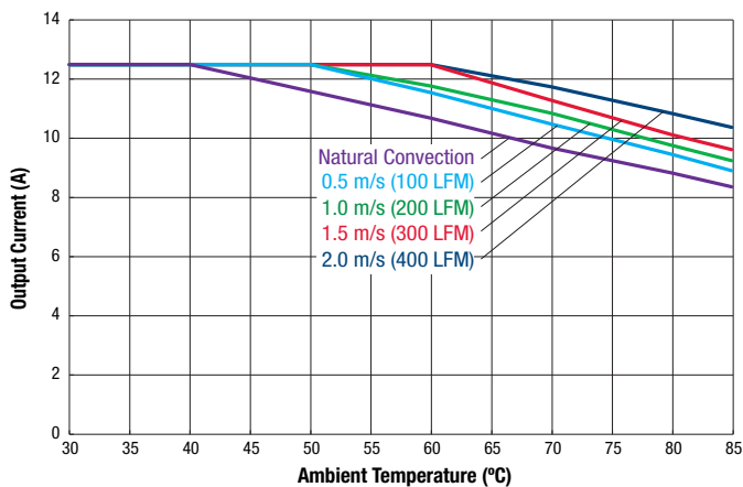
Maximum Current Temperature Derating at Sea Level (Vin = 75V, no baseplate. Airflow Direction Is Transverse from -Vin to +Vin.)
