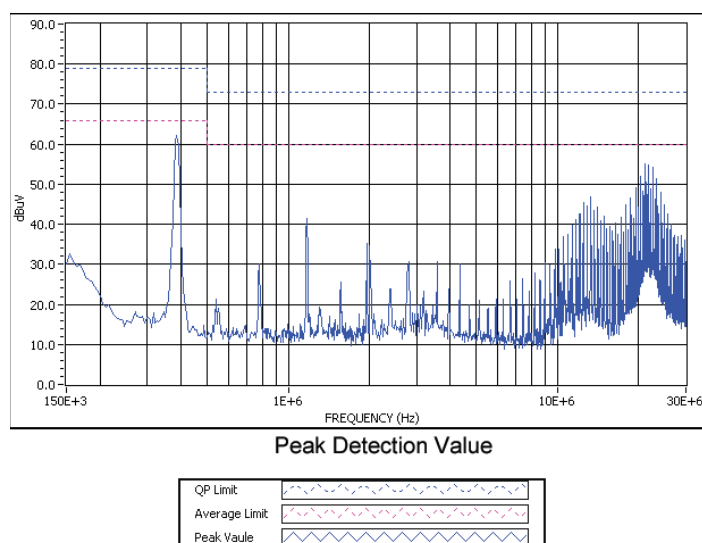
Graph 4. Conducted emissions performance, Negative Line, CISPR 22, Class A, 48 Vin, full load
