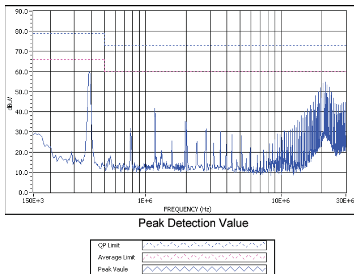
Graph 3. Conducted emissions performance, Positive Line, CISPR 22, Class A, 48 Vin, full load
