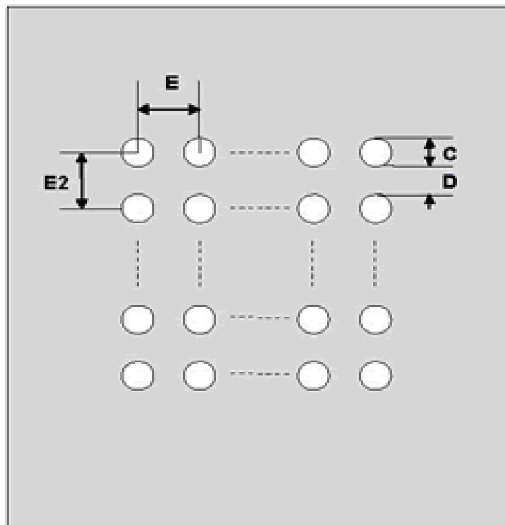
Top View (SMT Footprint)
