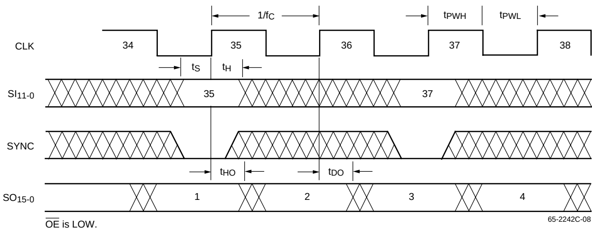
Figure 8. Interpolate Mode
