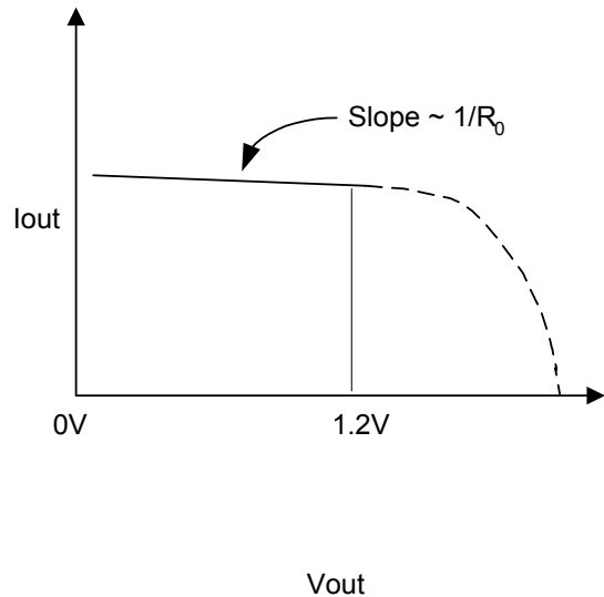
Figure 14. Buffer Characteristics
