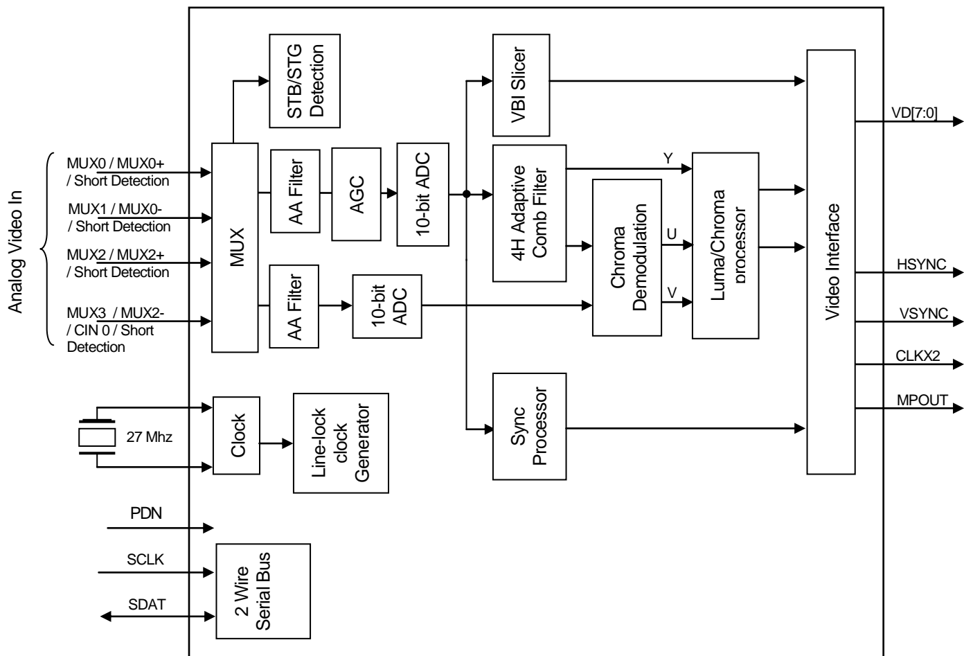
FIGURE 1. TW9990 BLOCK DIAGRAM
