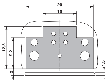
Dimensional drawing
