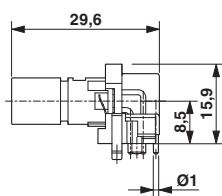
Dimensional drawing
