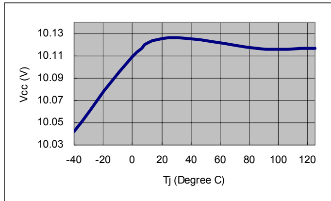
Vcc vs. Temp.
