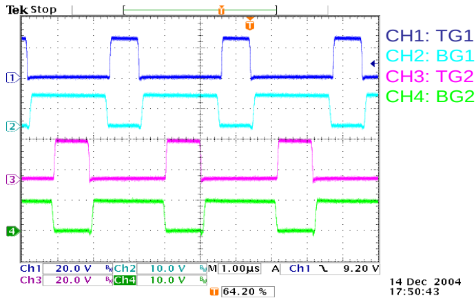
Gate waveform
