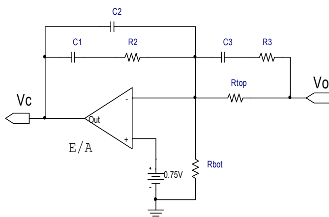
Fig. 12. Compensation network.
