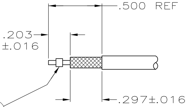
RECOMMENDED STRIP LENGTH FOR SOLDERED CENTER CONTACT
