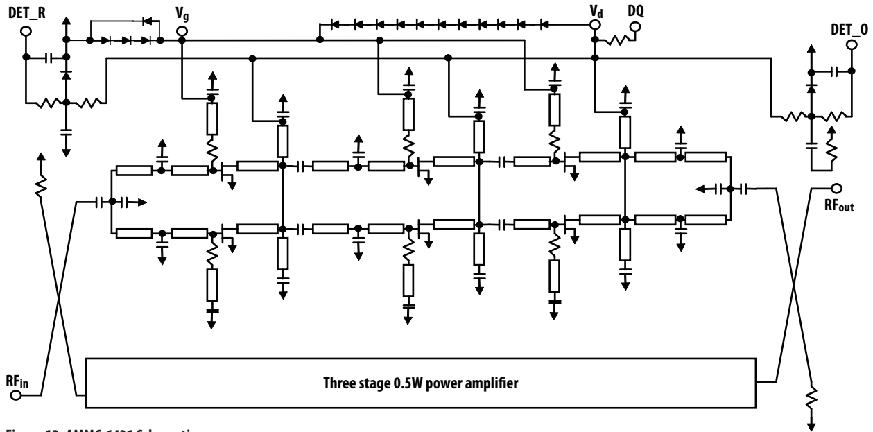
Figure 12. AMMC-6431 Schematic
