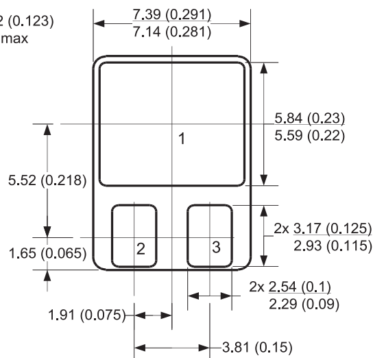
PACKAGE OUTLINE
