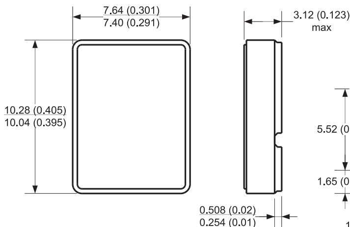
SMD-0.5/TO-276
