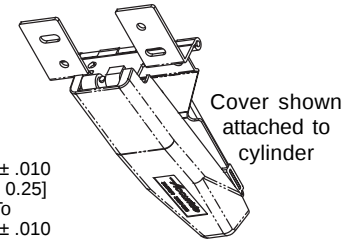
Cylinder Cover (Part Number 2336-2937-YE)
