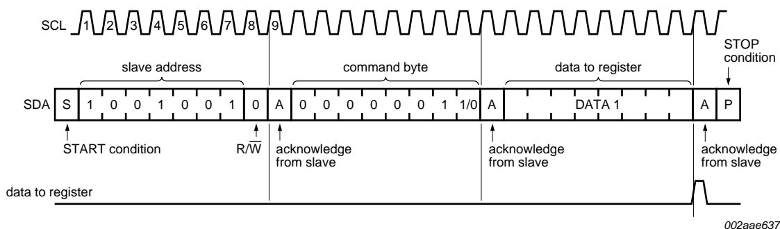
Fig 6. Write to configuration or polarity inversion registers
