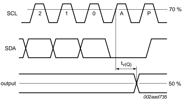
Fig 16. Expanded view of write to output port register
