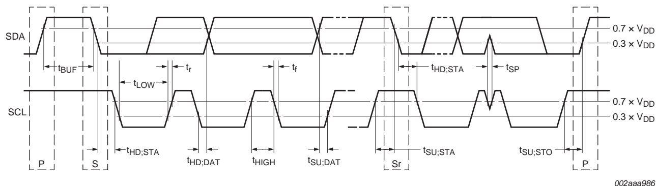
Fig 12. Definition of timing
