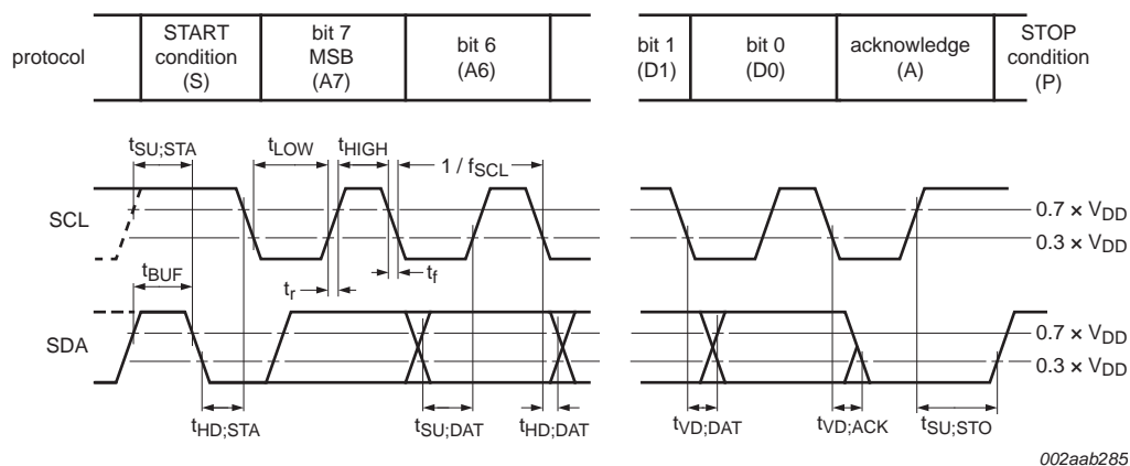
Fig 13. I 2 C-bus timing diagram
