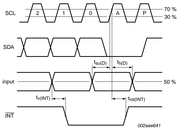
Fig 15. Expanded view of read input port register
