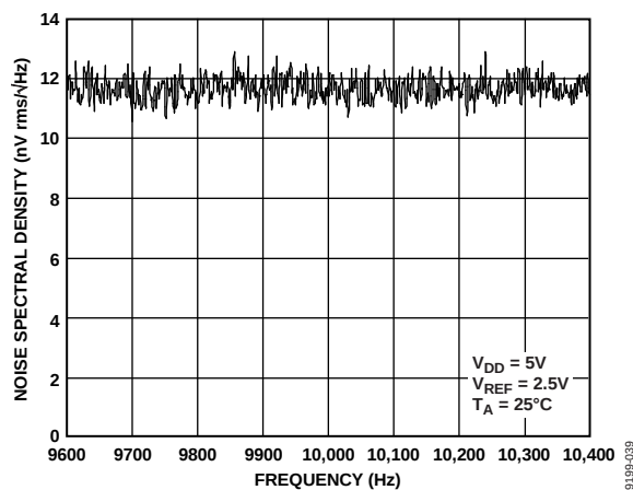
Figure 27. AD5512A/AD5542A Noise Spectral Density vs. Frequency, 10 kHz
