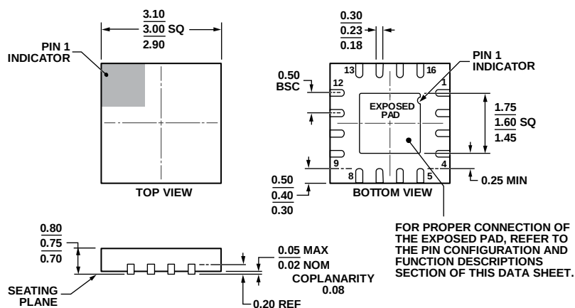
Figure 40. 16-Lead Lead Frame Chip Scale Package [LFCSP_WQ] 3 mm × 3 mm Body, Very Very Thin Quad (CP-16-22)
