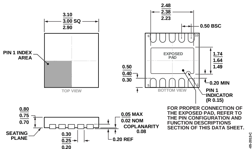
Figure 42. 10-Lead Lead Frame Chip Scale Package [LFCSP_WD] 3 mm × 3 mm Body, Very Very Thin, Dual Lead (CP-10-9)
