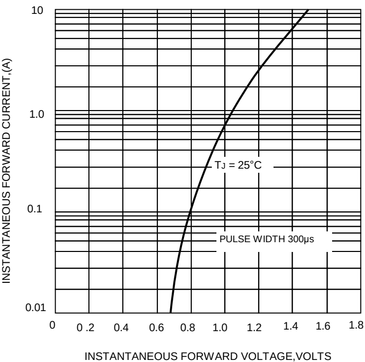
FIG.4-TYPICAL FORWARD CHARACTERISTICS
