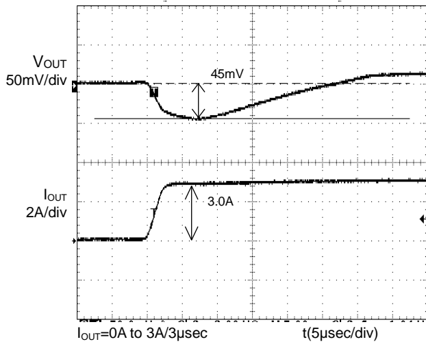
Figure 1. Transient Response (0A to 3A) C_{OUT}=150\mu\text{F} \times 2 , C_{FB}=0.01\mu\text{F}
