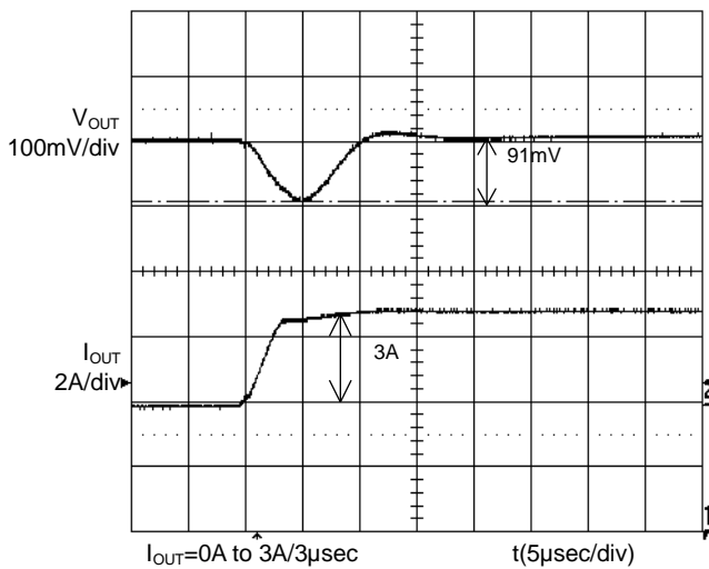
Figure 3. Transient Response (0A to 3A) C_{OUT}=47\mu\text{F} , C_{FB}=0.01\mu\text{F}
