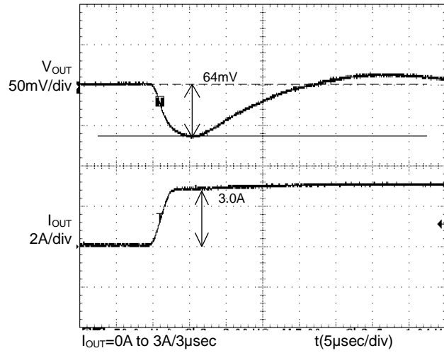
Figure 2. Transient Response (0A to 3A) C_{OUT}=150\mu\text{F}
