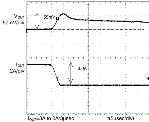
Figure 4. Transient Response (3A to 0A) C_{OUT}=150\mu\text{F} \times 2
