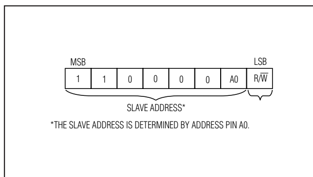
Figure 5. DS3514 Slave Address Byte
