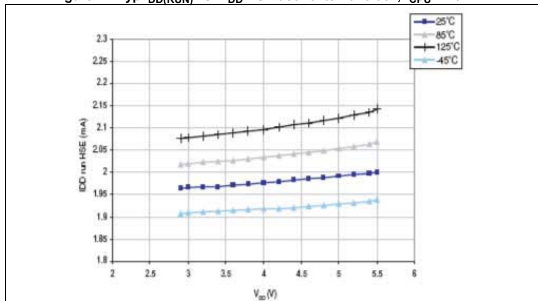
Figure 11. Typ I_{DD(RUN)} vs. V_{DD} HSE user external clock, f_{CPU} = 16 \text{ MHz}
