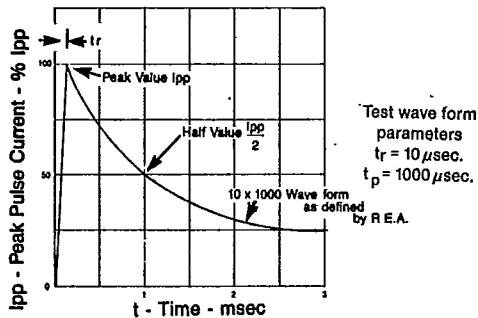
FIGURE 2 PULSE WAVEFORM
