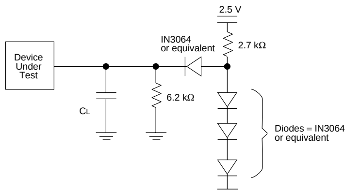
Figure 4 Test Conditions
