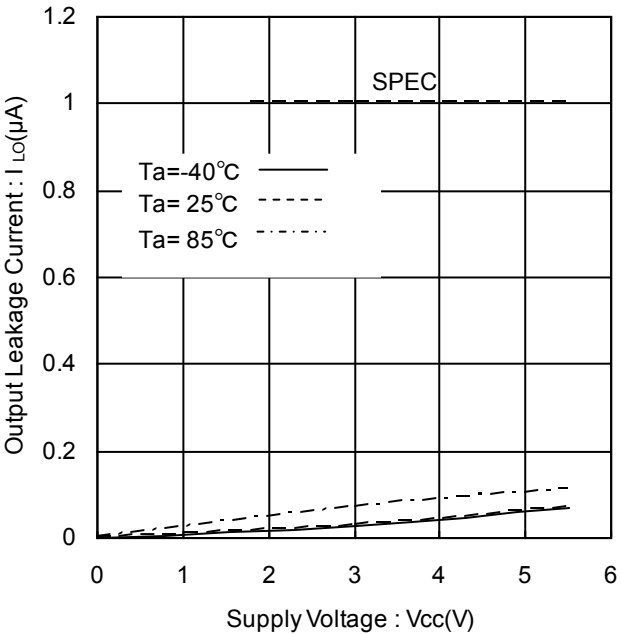
Figure 9. Output Leakage Current vs Supply Voltage (SDA)
