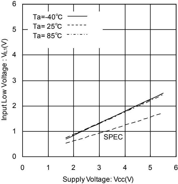
Figure 5. Input Low Voltage1,2 vs Supply Voltage (A0, A1, A2, SCL, SDA, WP)
