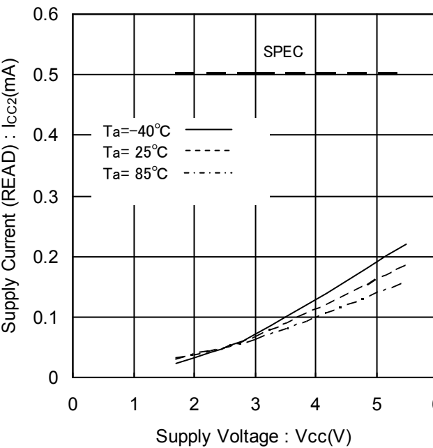
Figure 11. Supply Current (READ) vs Supply Voltage (f SCL =400kHz)
