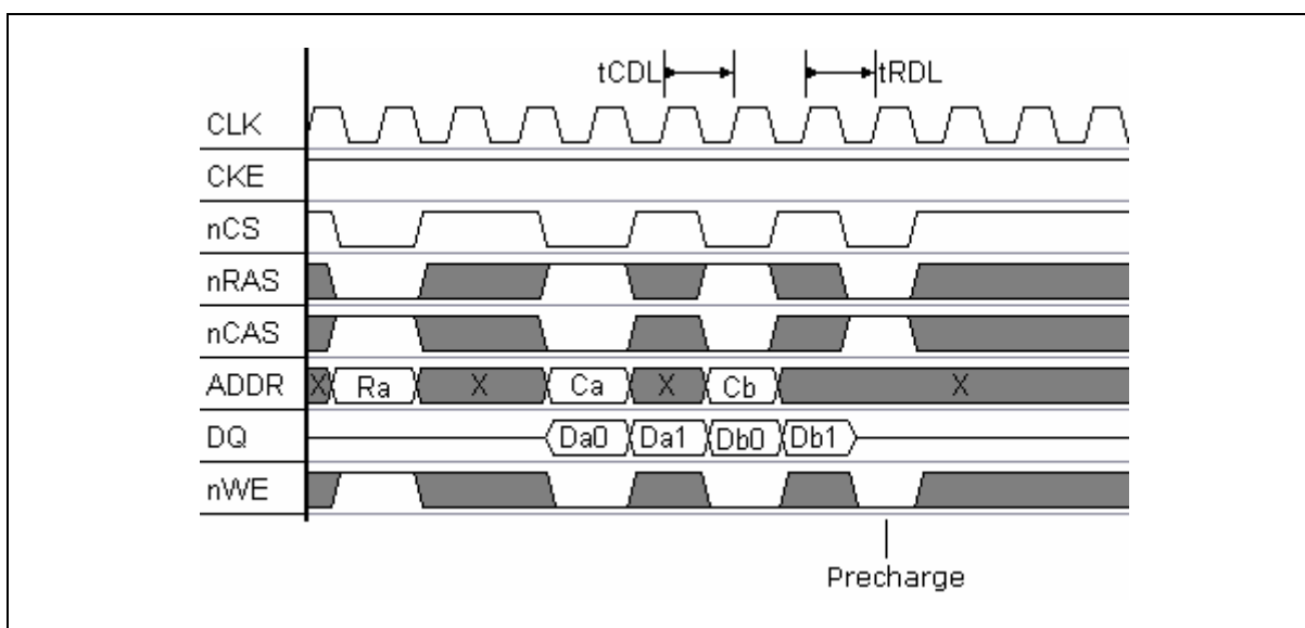
Fig 7.3.5 Access timing 2 of SDRAM
