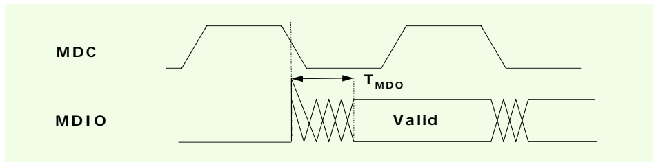
MDIO Write to PHY Timing
