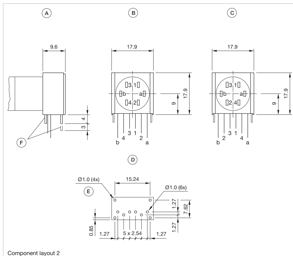
Component layout 2
