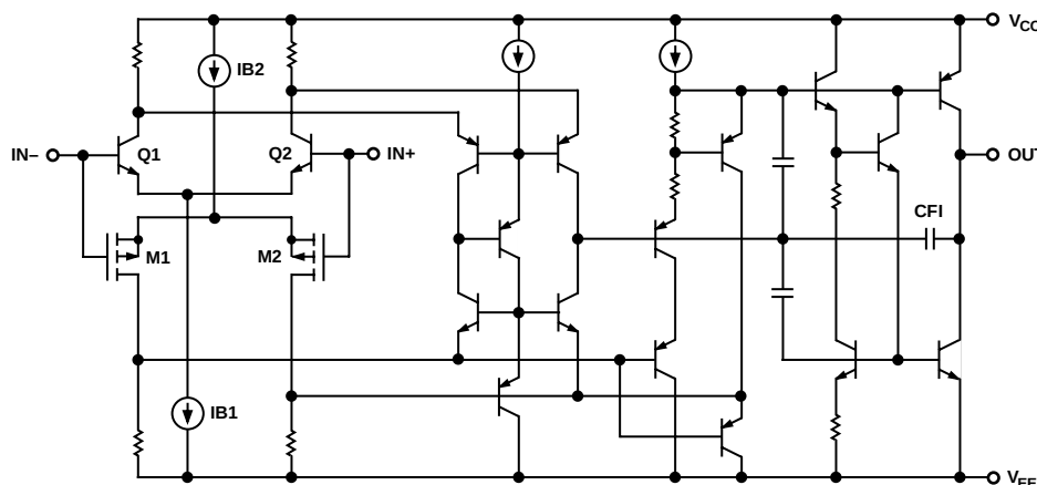
Figure 27. Simplified Schematic
