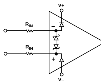
Figure 28. Using Resistors for Input Overcurrent Protection
