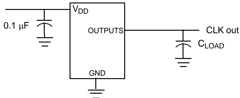
Figure 7. Test Circuit
