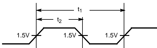
Figure 2. Duty Cycle Timing
