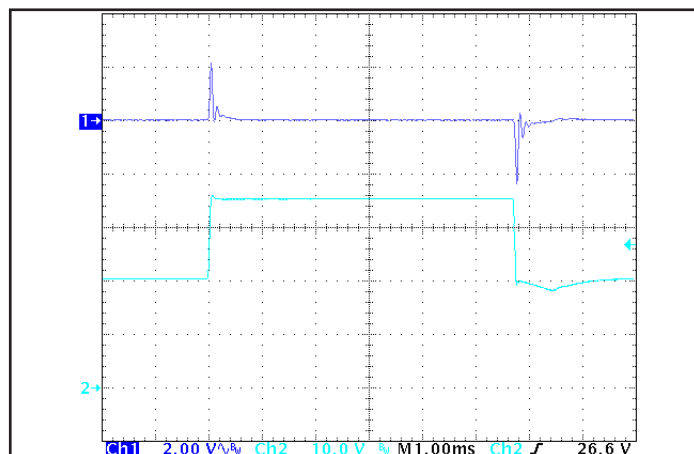
Figure 6: Output voltage response to step-change in input voltage (Vnom.-Vmax-Vnom.), at Max. load current. Load cap: 1μF ceramic cap. Ch 1: Vout, Ch 2: Vin.
