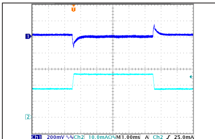
Figure 5: Output voltage response to step-change in load current (50%-75%-50% of Iout(max); dI/dt = 0.1A/us). Load cap: 15μF tantalum cap and 1μF ceramic cap. Ch 1: Vout, Ch 2: Iout.
