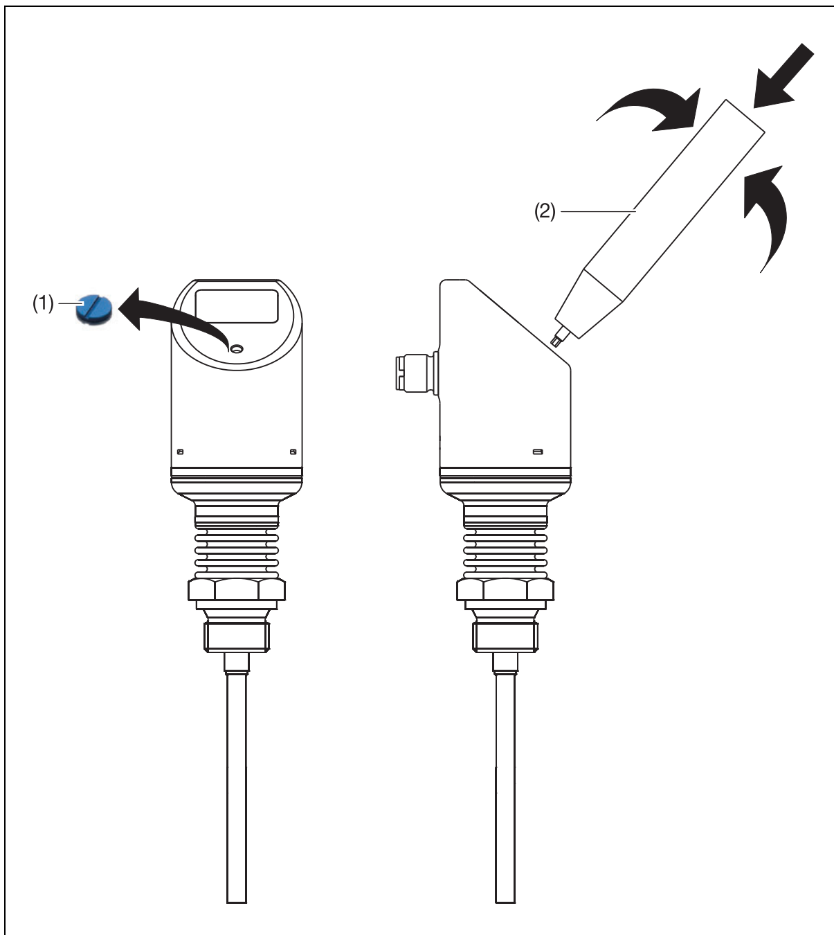
(1) Locking screw
