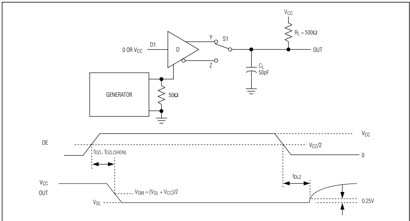
Figure 5. Driver Enable and Disable Times ( t_{DLZ} , t_{DLH} , t_{DLH(SHDN)} )
