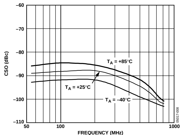
Figure 2. Composite Second-Order vs. Frequency
